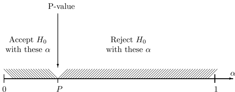
FIGURE 9.11: P -value separates \alpha -to-accept and \alpha -to-reject.
